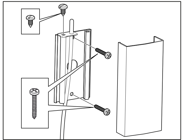
Figure 11: Installing the sensor, single heater
