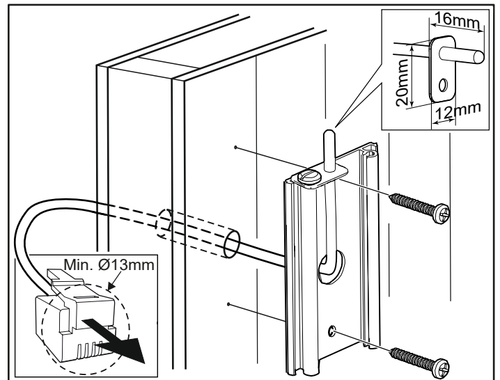
Figure 12: Wiring through the wall.
