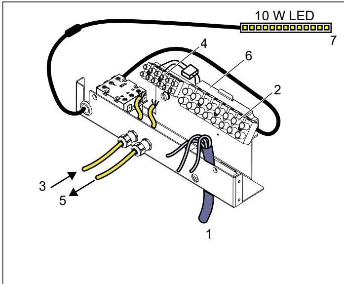
Figure 9: Electrical Compartment
