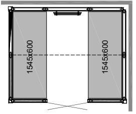
PANACEA 2117 2B Size: 2125 x 1725 x 2090 mm
