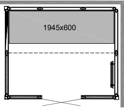
PANACEA 2117 1B Size: 2125 x 1725 x 2090 mm
