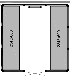
PANACEA 2525 2B Size: 2525 x 2525 x 2090 mm
