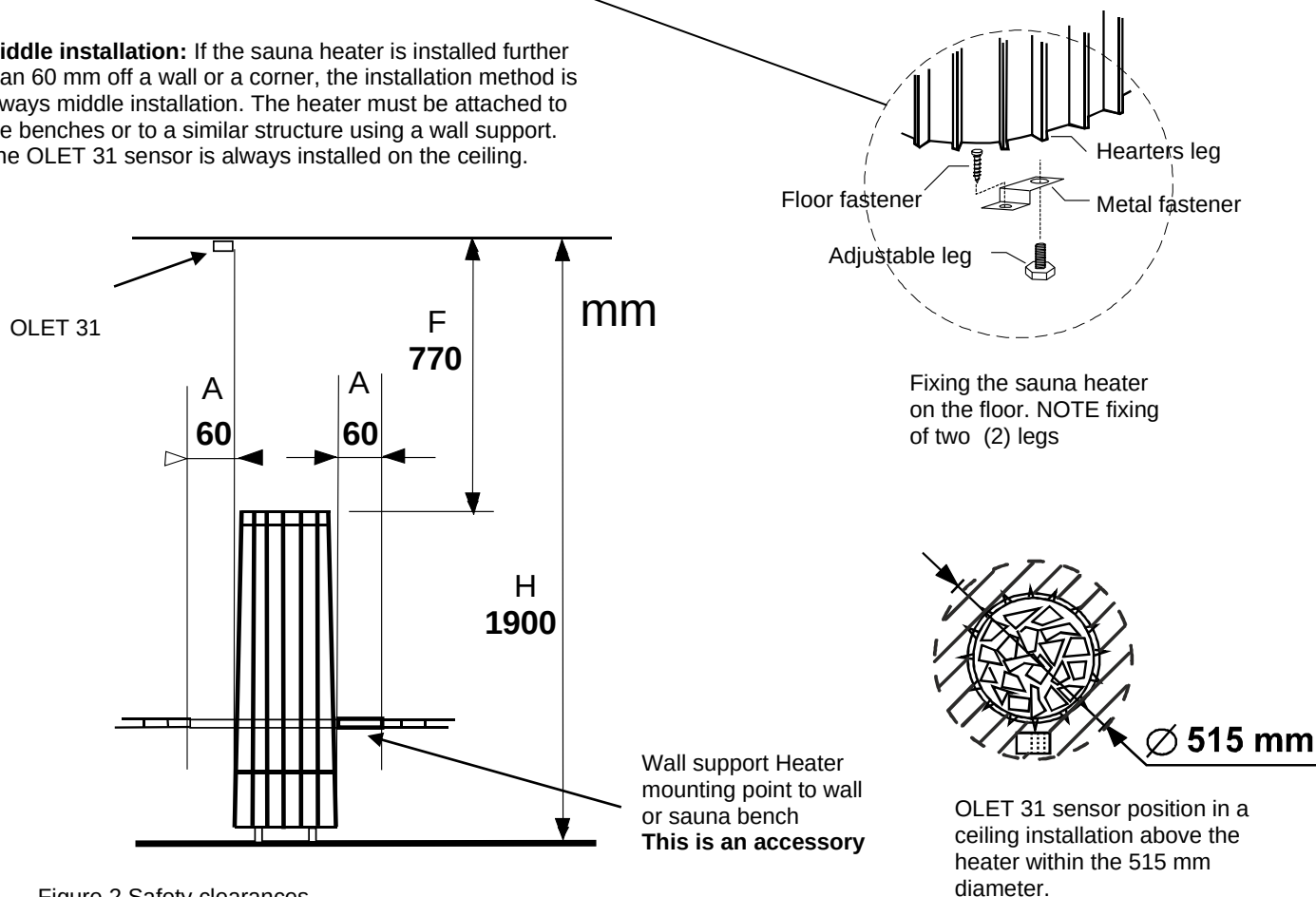
Figure 2 Safety clearances
