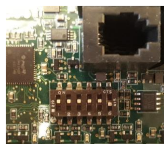
Figure 6 DIP switch positions for using a heater
