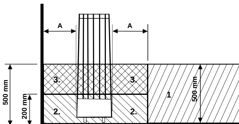
Figure 5 Location for the connection box
