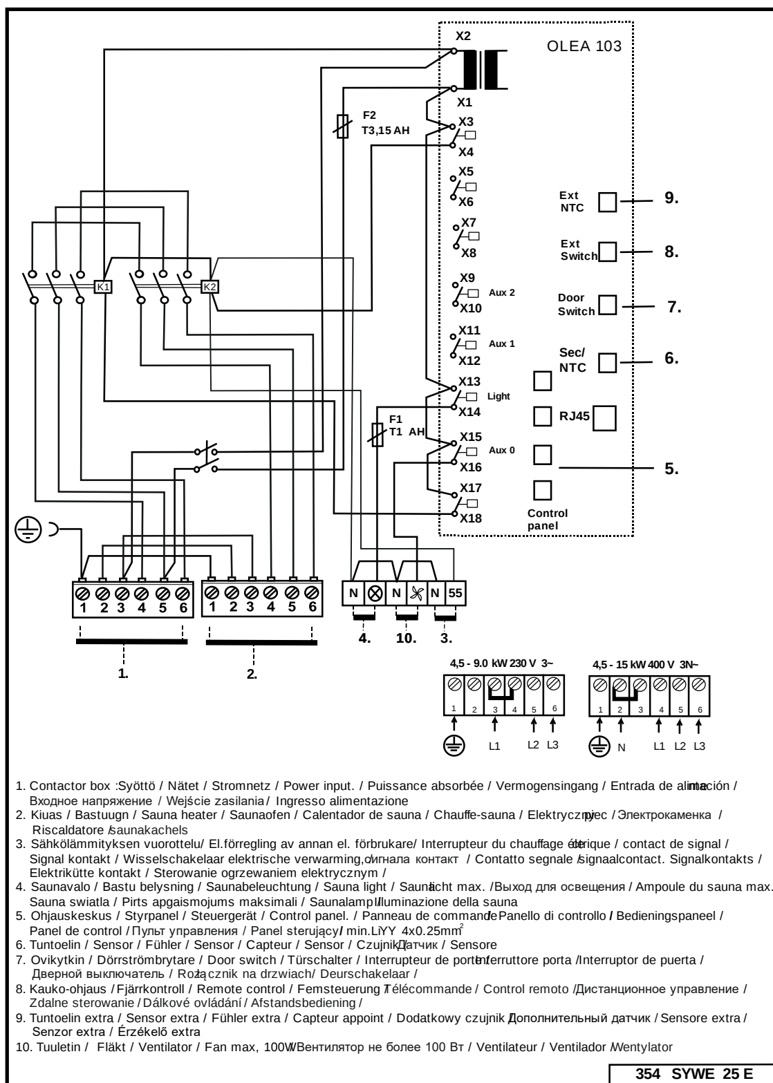
Figure 4 Wiring diagram for contactor box WE 40
