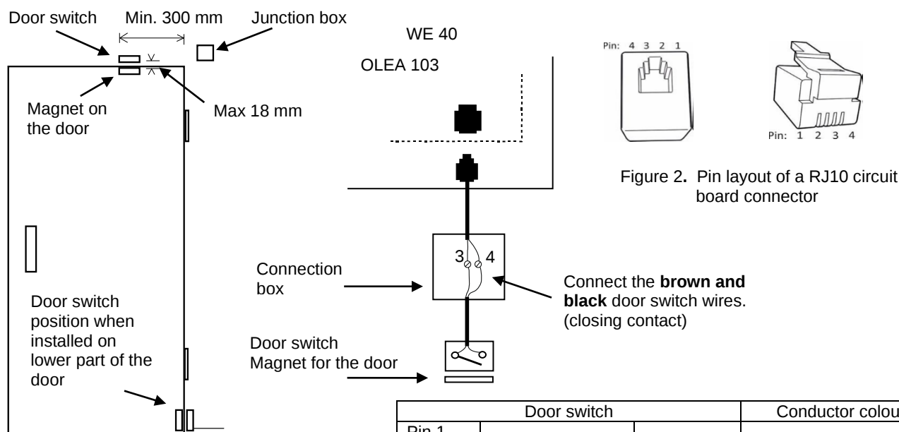
Figure 3. Installing the door switch
